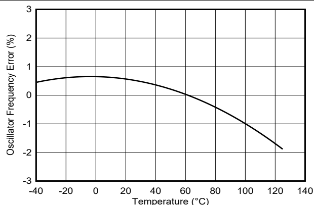
Figure 6-11. Oscillator Frequency Error vs Temperature
