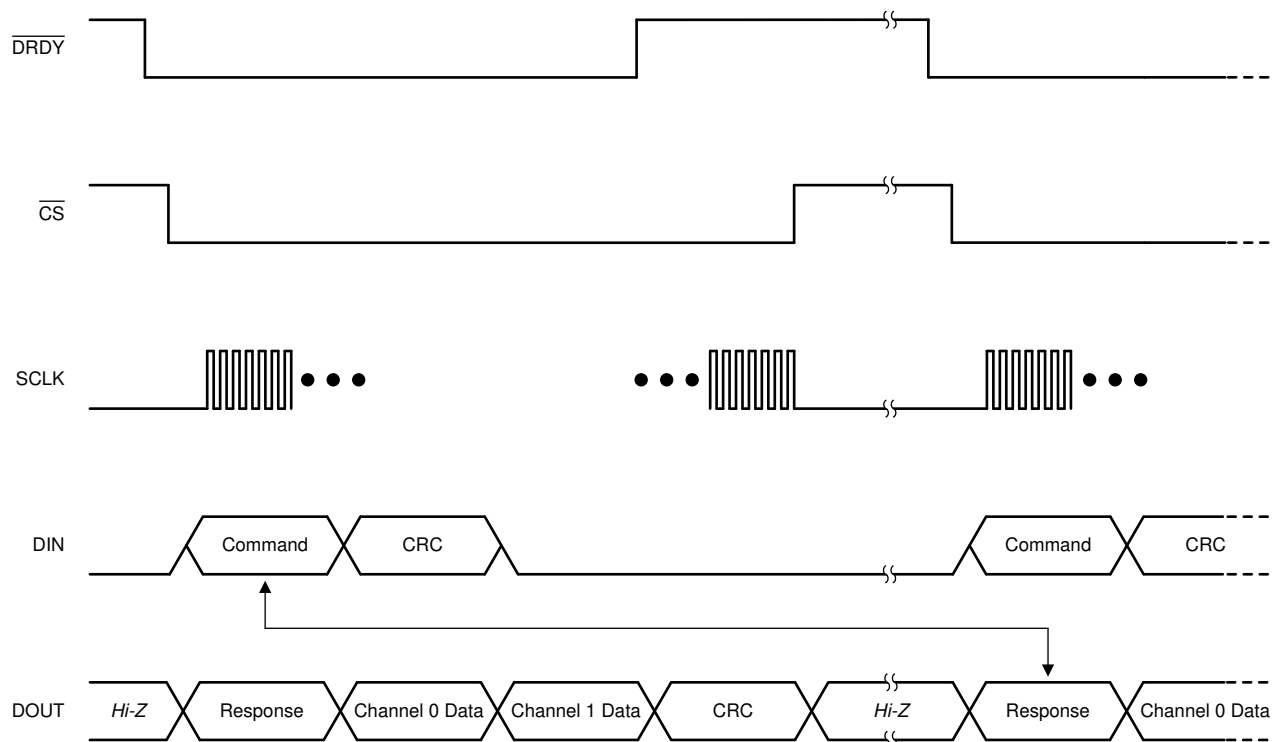
Figure 8-14. Typical Communication Frame
