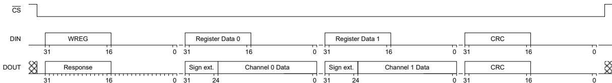
Figure 8-17. SPI Frame using 32-bit, sign-extended Word Size
