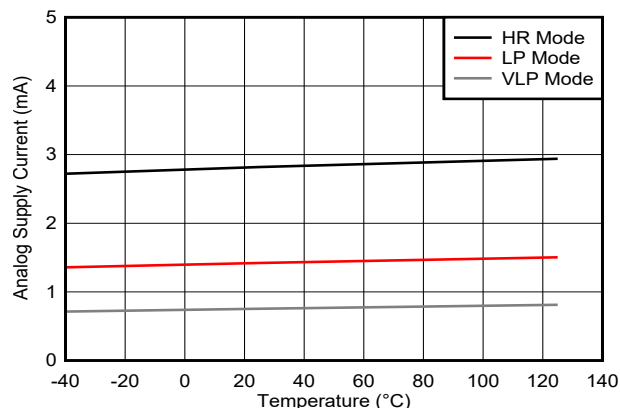
Figure 6-12. Analog Supply Current vs Temperature
