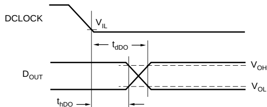
Voltage Waveforms for D_{OUT} Delay Times, t_{dDO}
