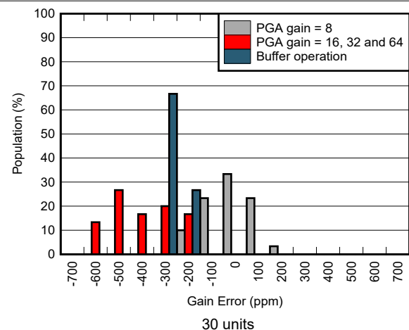
Figure 5-42. Gain Error Distribution
