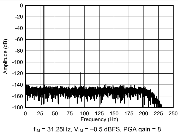
Figure 5-17. High-Power Mode FFT Spectrum
