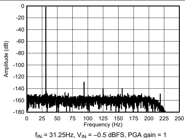
Figure 5-30. Low-Power Mode FFT Spectrum
