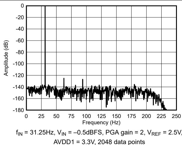
Figure 5-32. Low-Power Mode FFT Spectrum
