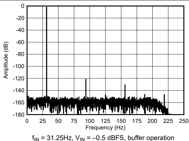
Figure 5-15. High-Power Mode FFT Spectrum
