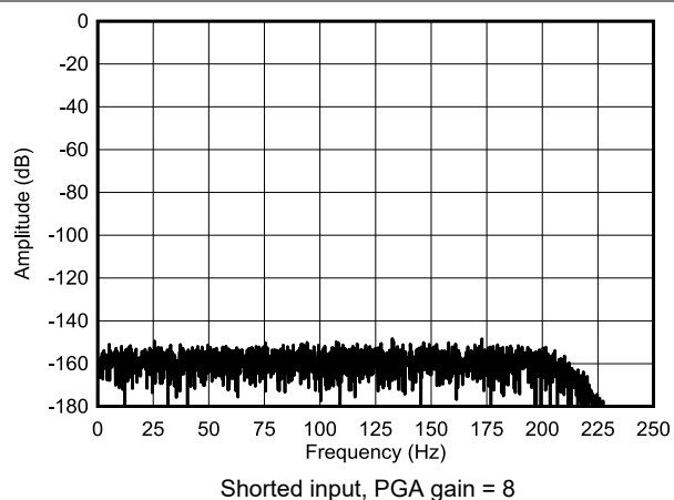
Figure 5-28. Low-Power Mode FFT Spectrum
