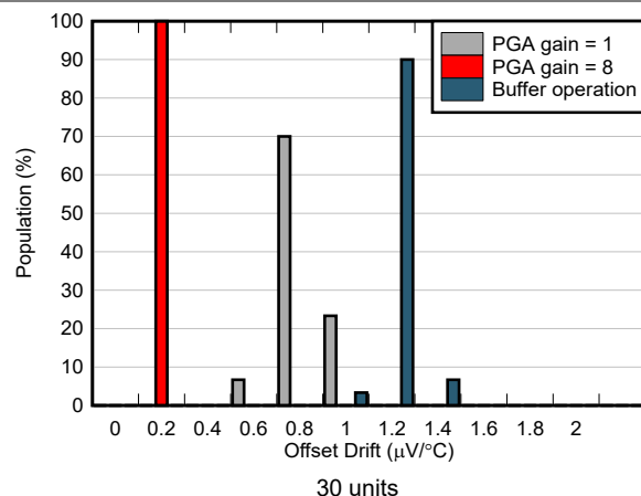
Figure 5-40. Offset Drift Distribution
