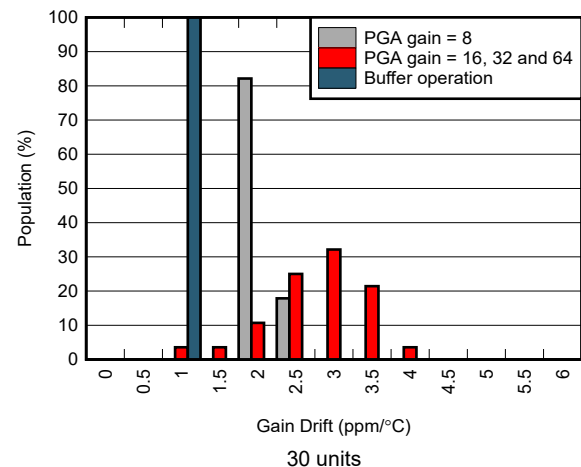
Figure 5-44. Gain Drift Distribution
