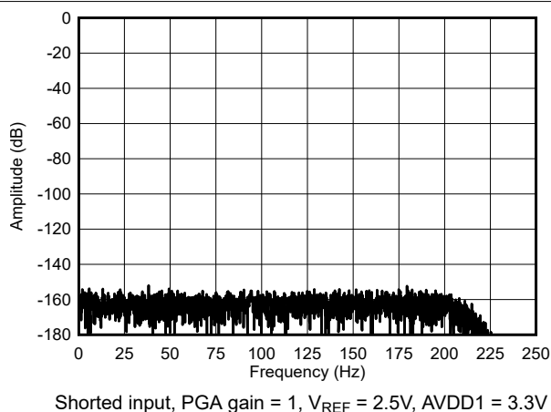
Figure 5-29. Low-Power Mode FFT Spectrum
