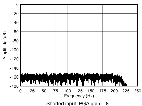
Figure 5-20. Mid-Power Mode FFT Spectrum
