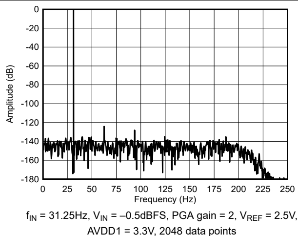
Figure 5-16. High-Power Mode FFT Spectrum
