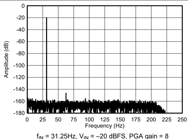
Figure 5-18. High-Power Mode FFT Spectrum
