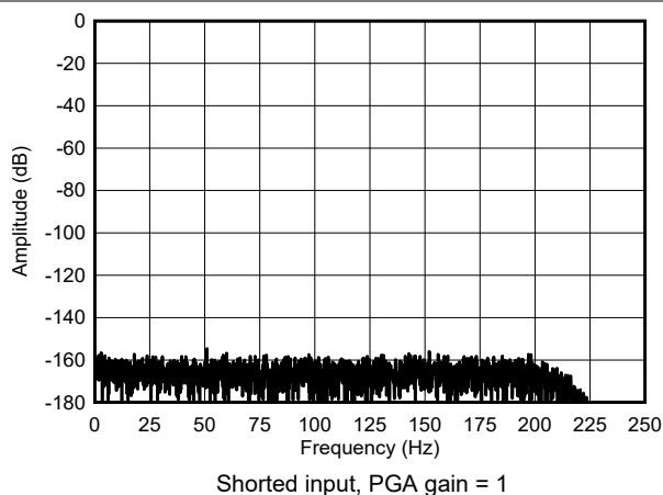
Figure 5-27. Low-Power Mode FFT Spectrum
