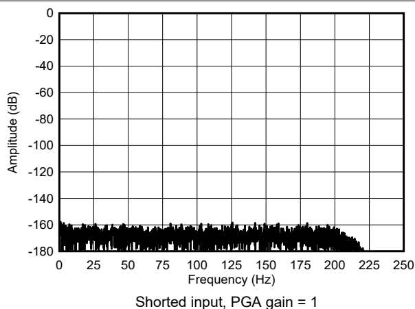
Figure 5-19. Mid-Power Mode FFT Spectrum
