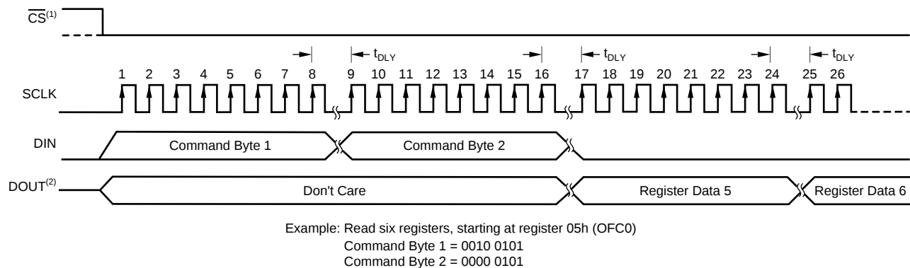
Figure 60. Read Register Data (Table 24 shows t_{DLY} )
