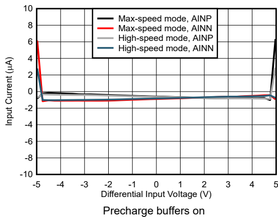
Figure 5-41. Input Current vs Differential Voltage
