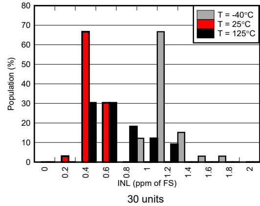
Figure 5-68. INL Over-Temperature Distributions
