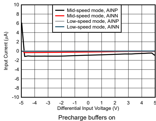
Figure 5-42. Input Current vs Differential Voltage
