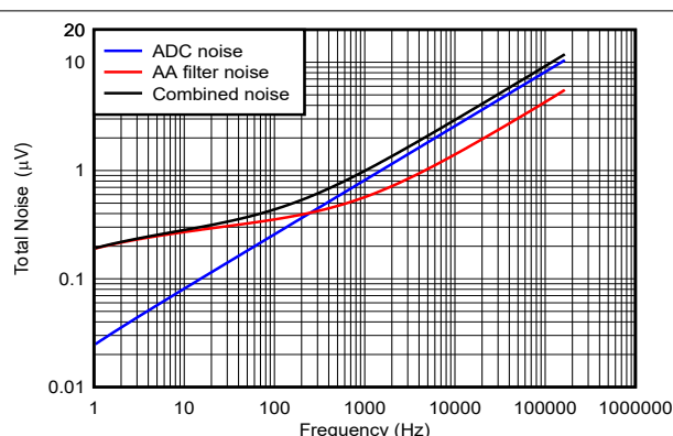
Figure 9-12. Total Noise
