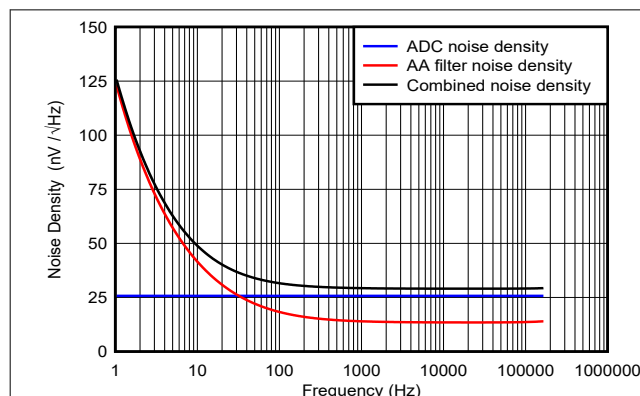
Figure 9-11. Noise Density
