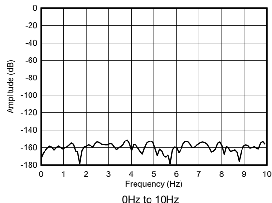
Figure 5-26. Low-Speed Mode, Shorted-Input FFT
