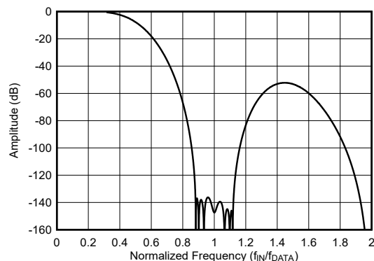
Figure 7-11. FIR1 Filter Frequency Response (OSR = 32)
