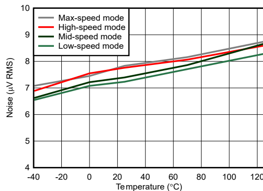
Figure 5-38. Noise Performance vs Temperature
