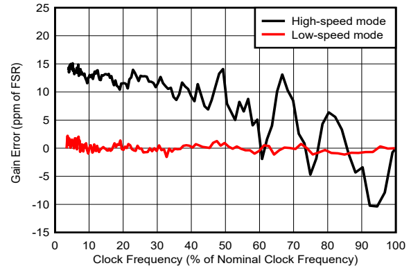
Figure 5-56. Gain Error vs Clock Frequency
