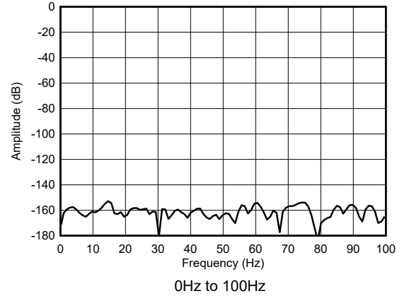
Figure 5-8. Max-Speed Mode, Shorted-Input FFT
