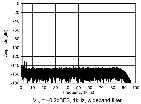
Figure 5-24. Mid-Speed Mode, Full-Scale FFT
