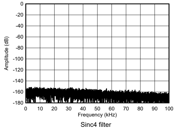
Figure 5-22. Mid-Speed Mode, Shorted-Input FFT
