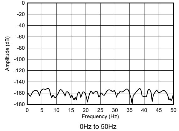
Figure 5-20. Mid-Speed Mode, Shorted-Input FFT
