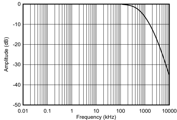
Figure 9-7. PGA855 Antialias Filter Response
