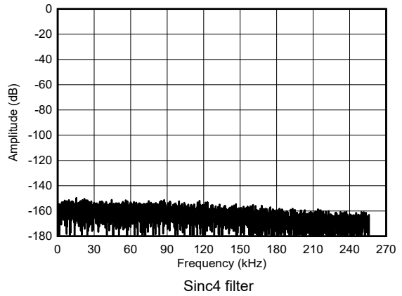
Figure 5-10. Max-Speed Mode, Shorted-Input FFT
