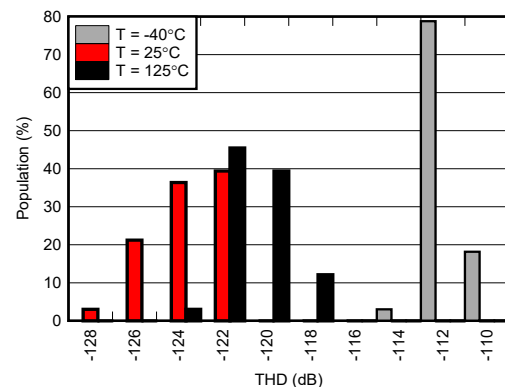
Figure 5-58. THD Distribution
