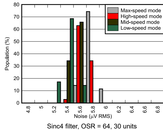
Figure 5-36. Noise Performance Distributions
