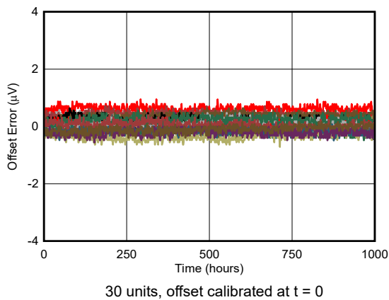
Figure 5-51. Long-Term Offset Drift
