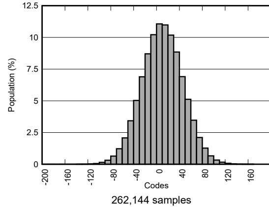
Figure 5-32. High-Speed Mode Code Distributions
