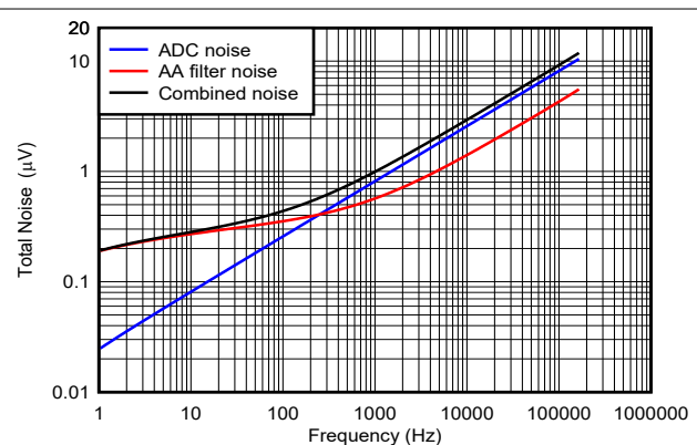
Figure 9-5. Total Noise
