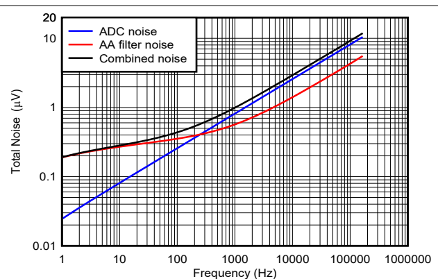
Figure 9-5. Total Noise
