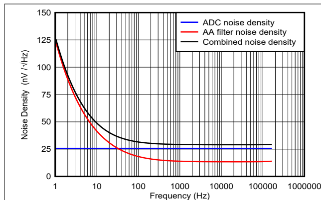
Figure 9-4. Noise Density
