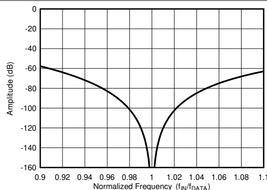
Figure 8-18. Detail Sinc3 Frequency Response (OSR = 32000)
