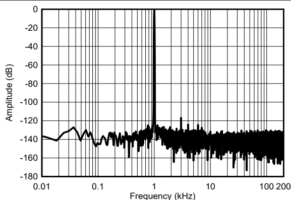
Figure 6-14. Shorted Input FFT
