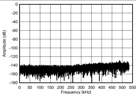
Figure 6-12. Shorted Input FFT
