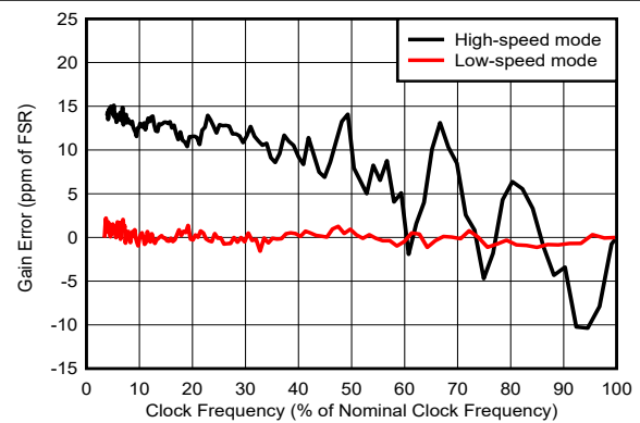
Gain error calibrated at nominal clock frequency Figure 6-33. Gain Error vs Clock Frequency
