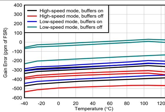
N = 3 Figure 6-32. Gain Error vs Temperature
