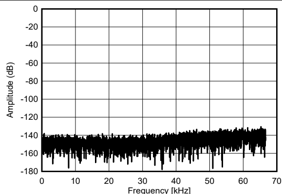
Figure 6-13. Shorted Input FFT
