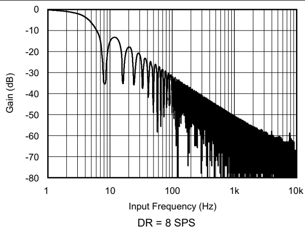
Figure 6-21. Digital Filter Frequency Response
