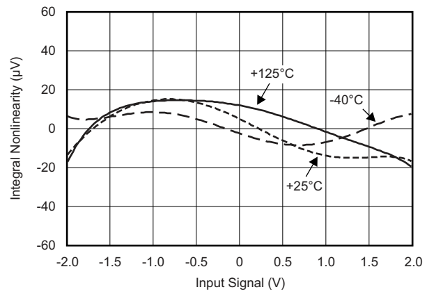
Figure 6-9. INL vs Input Signal
