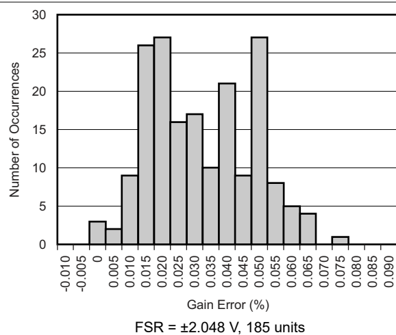
Figure 6-17. Gain Error Histogram
