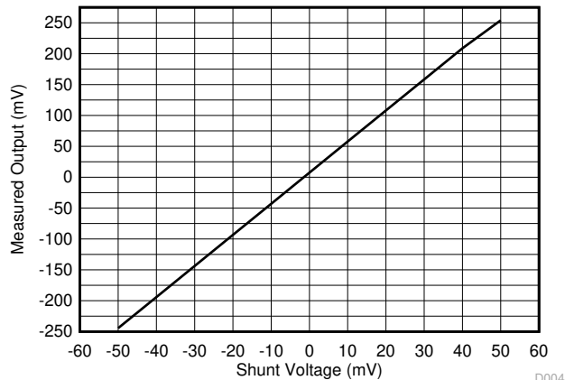
Figure 9-7. Measured Output vs Shunt Voltage ( V_{SHUNT} )
