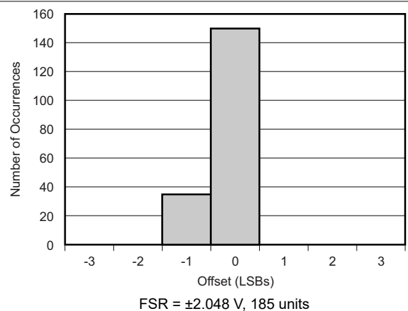
Figure 6-18. Offset Histogram
