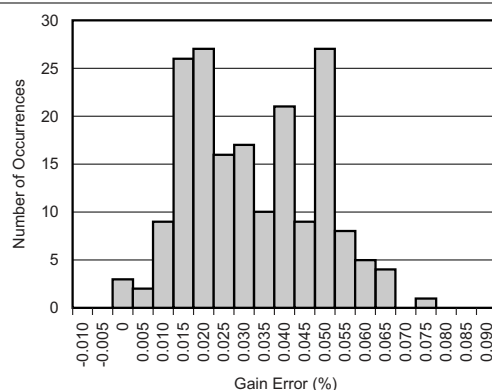
Figure 6-3. Gain Error Histogram
