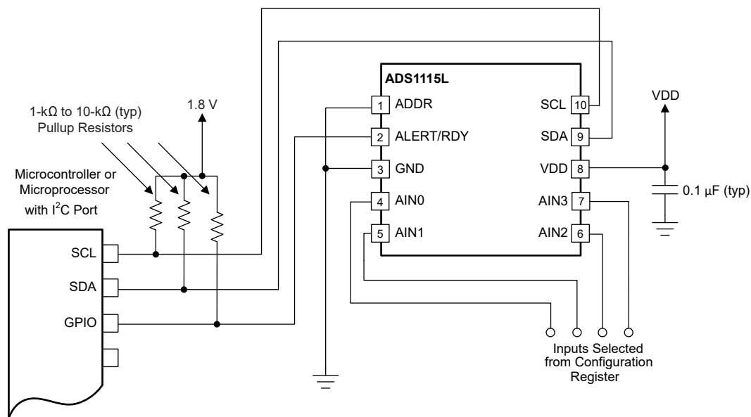
Figure 10-1. Typical Connections of the ADS1115L
