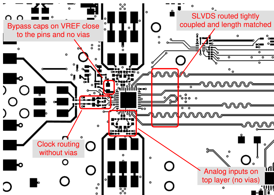
Figure 9-10. Layout example: top layer of ADC366x EVM
