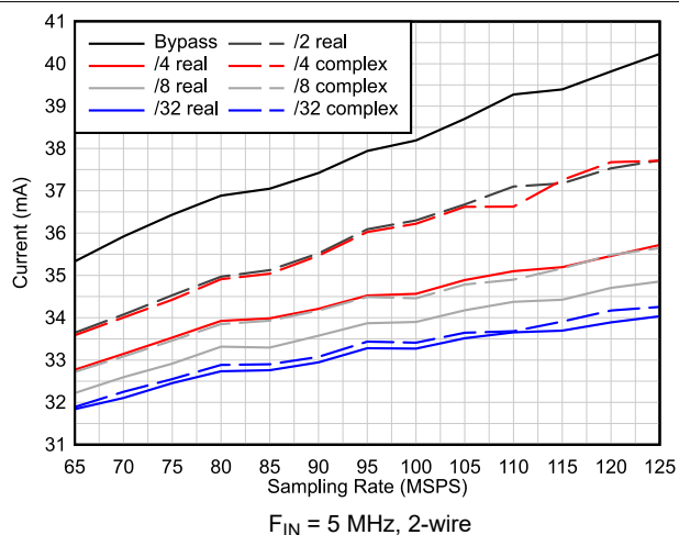
Figure 6-28. Power Consumption vs Decimation
