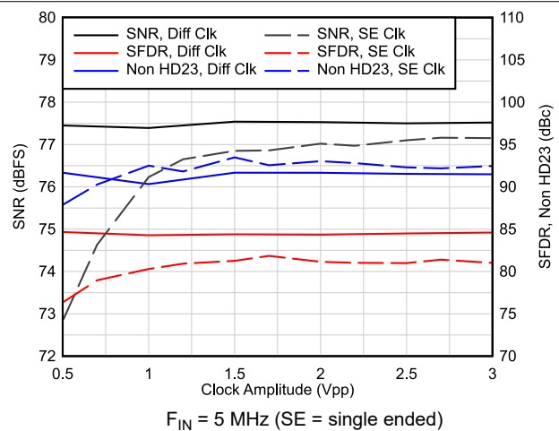
Figure 6-18. AC Performance vs Clock Amplitude
