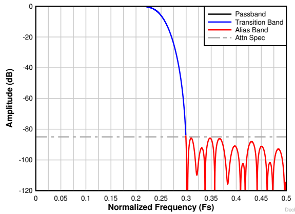
Figure 8-21. Decimation by 2 complex frequency response
