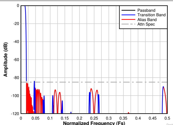
Figure 8-29. Decimation by 32 complex frequency response
