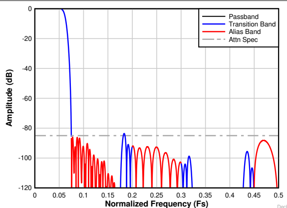
Figure 8-25. Decimation by 8 complex frequency response
