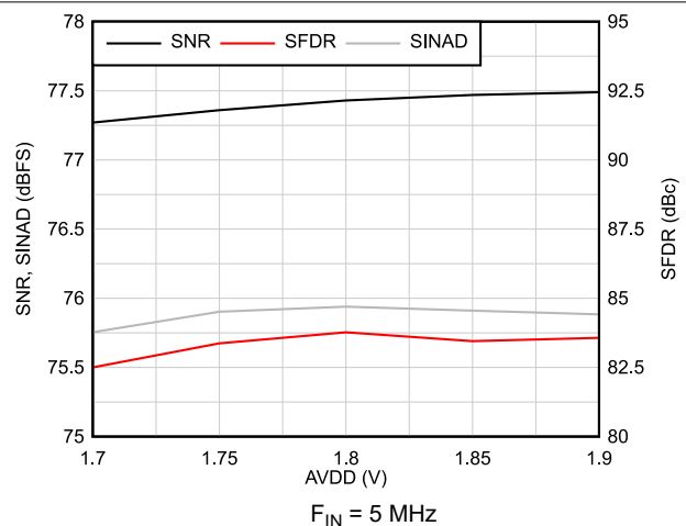
Figure 6-20. AC Performance vs AVDD
