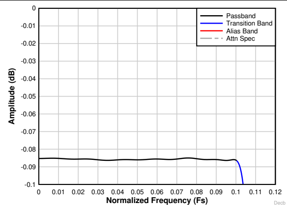
Figure 8-24. Decimation by 4 complex passband ripple response
