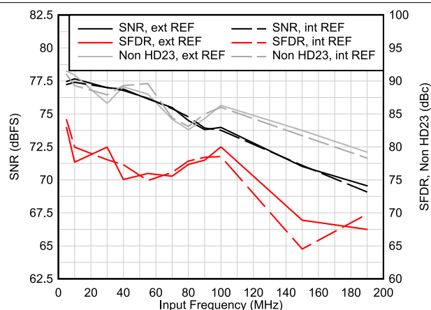
Figure 6-13. AC Performance vs Input Frequency
