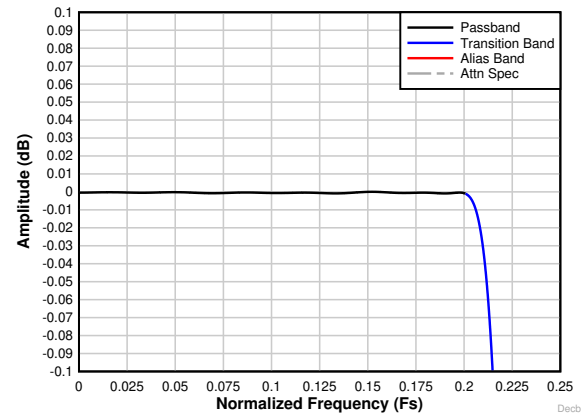
Figure 8-22. Decimation by 2 complex passband ripple response
