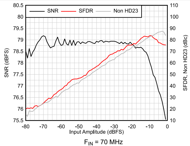
Figure 6-16. AC Performance vs Input Amplitude
