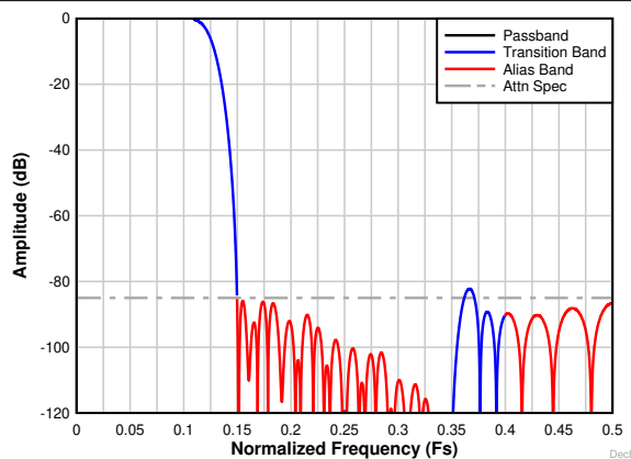
Figure 8-23. Decimation by 4 complex frequency response
