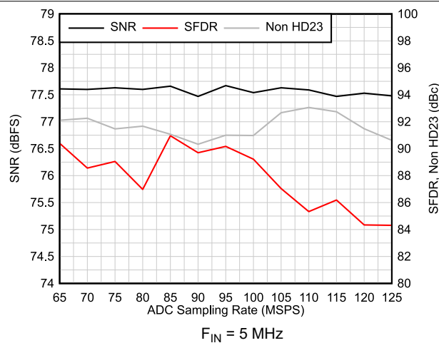
Figure 6-17. AC Performance vs Sampling Rate
