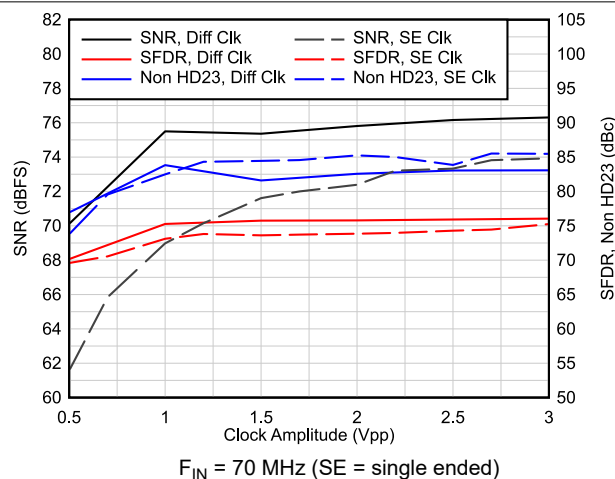
Figure 6-19. AC Performance vs Clock Amplitude
