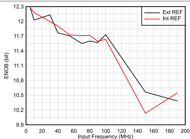
Figure 6-14. ENOB vs Input Frequency
