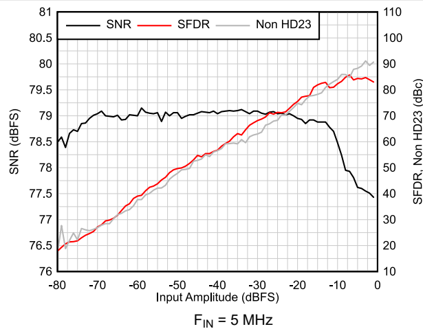
Figure 6-15. SNR, SFDR vs Input Amplitude
