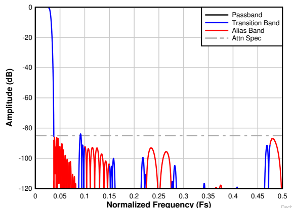
Figure 8-27. Decimation by 16 complex frequency response
