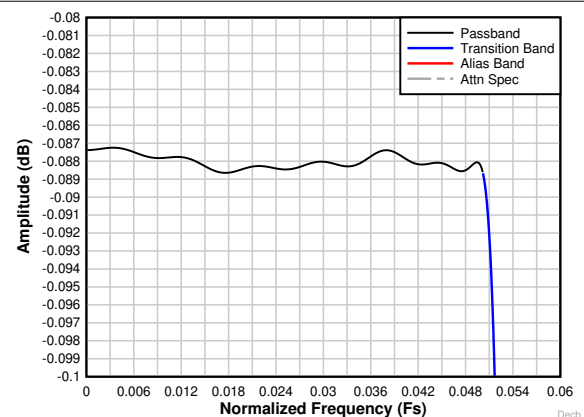
Figure 8-26. Decimation by 8 complex passband ripple response
