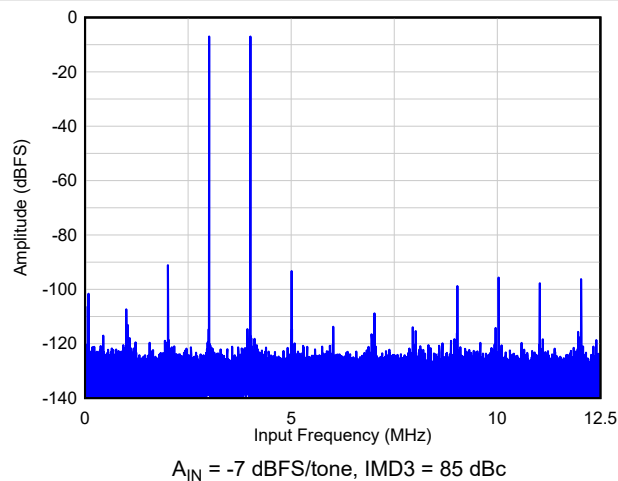
Figure 6-24. Two Tone FFT at F_{IN} = 3/4\text{ MHz}
