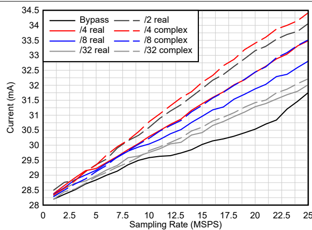
Figure 6-38. I_{OVDD} Current vs Decimation
