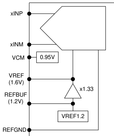
Figure 8-17. Different voltage reference options for ADC366x
