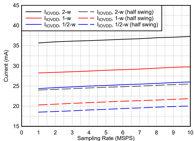
Figure 6-17. I_{OVDD} Current vs Interface
