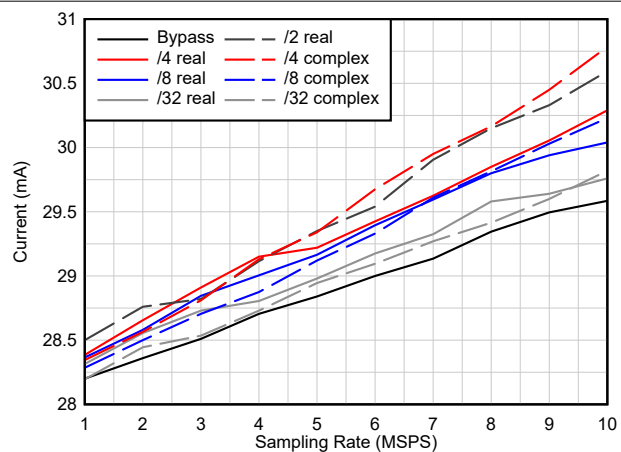
Figure 6-16. I_{OVDD} Current vs Decimation
