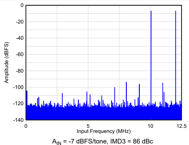
Figure 6-25. Two Tone FFT at F_{IN} = 10/12\text{ MHz}
