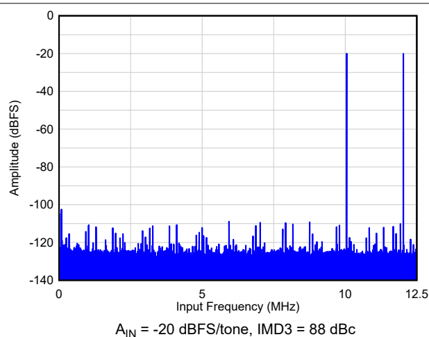
Figure 6-26. Two Tone FFT at F_{IN} = 10/12\text{ MHz}
