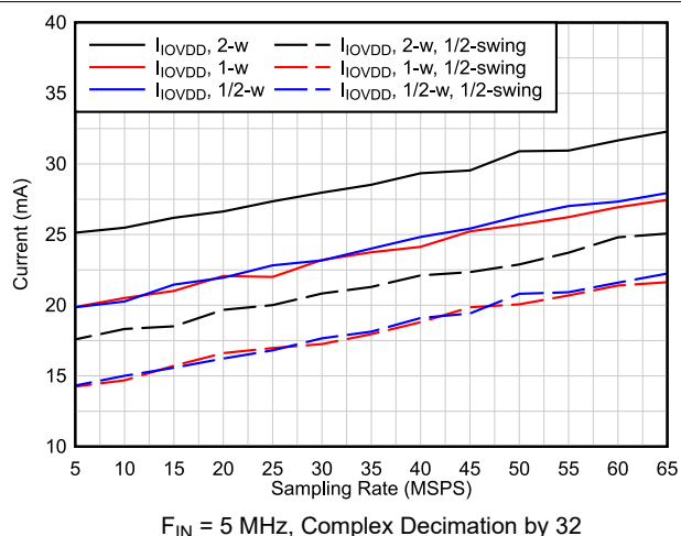
Figure 6-65. IOVDD Current vs Output Interface
