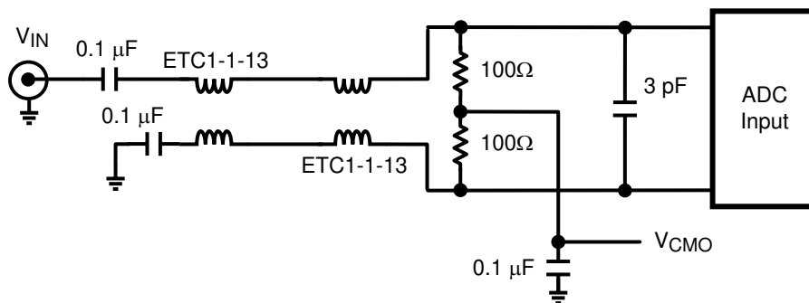
Figure 21. High Input Frequency Transformer Drive Circuit
