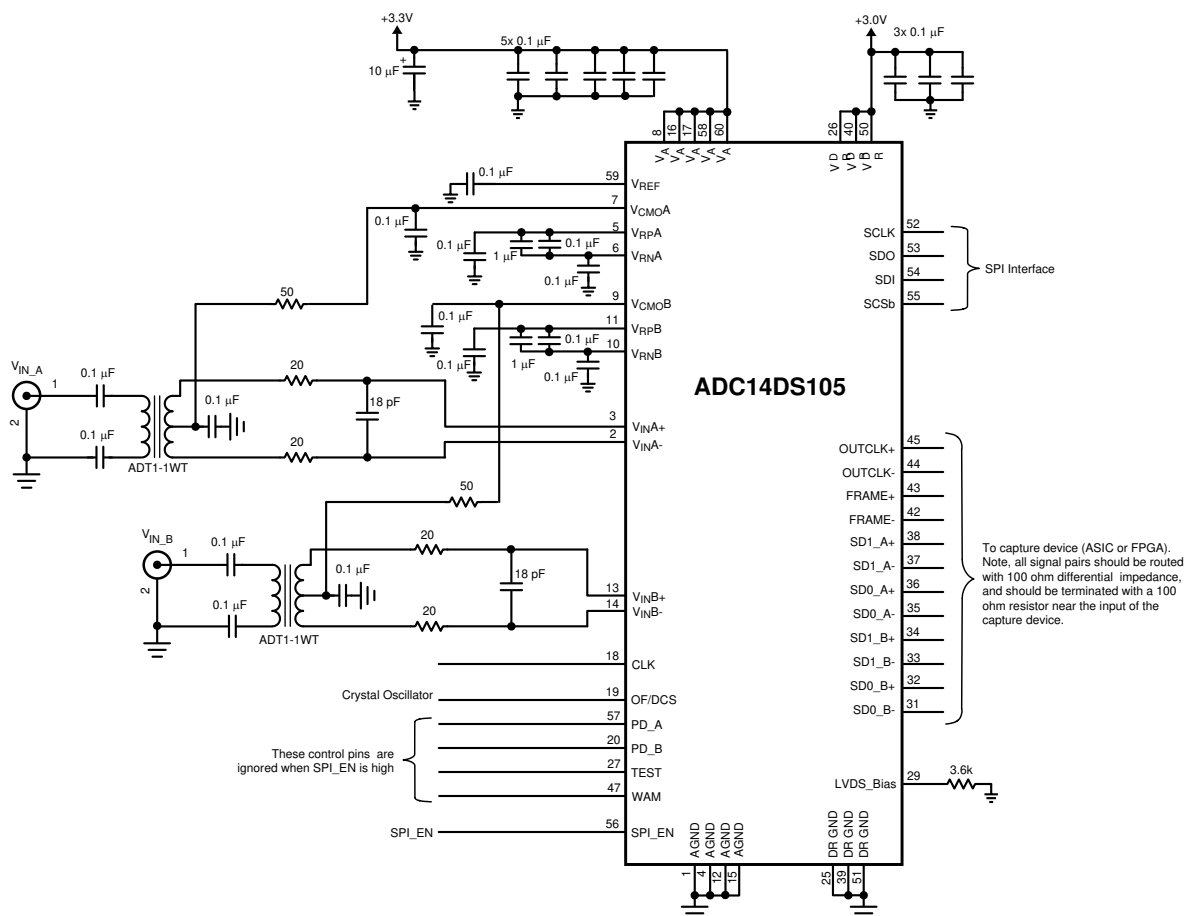
Figure 22. Application Circuit
