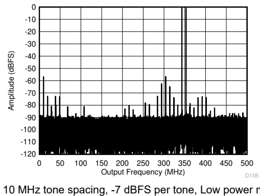
10 MHz tone spacing, -7 dBFS per tone, Low power mode, 1000MSPS
