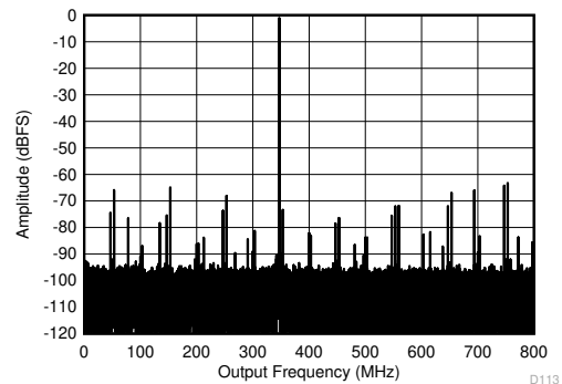
Figure 5-6. Single Tone FFT at 347 MHz and -1 dBFS
