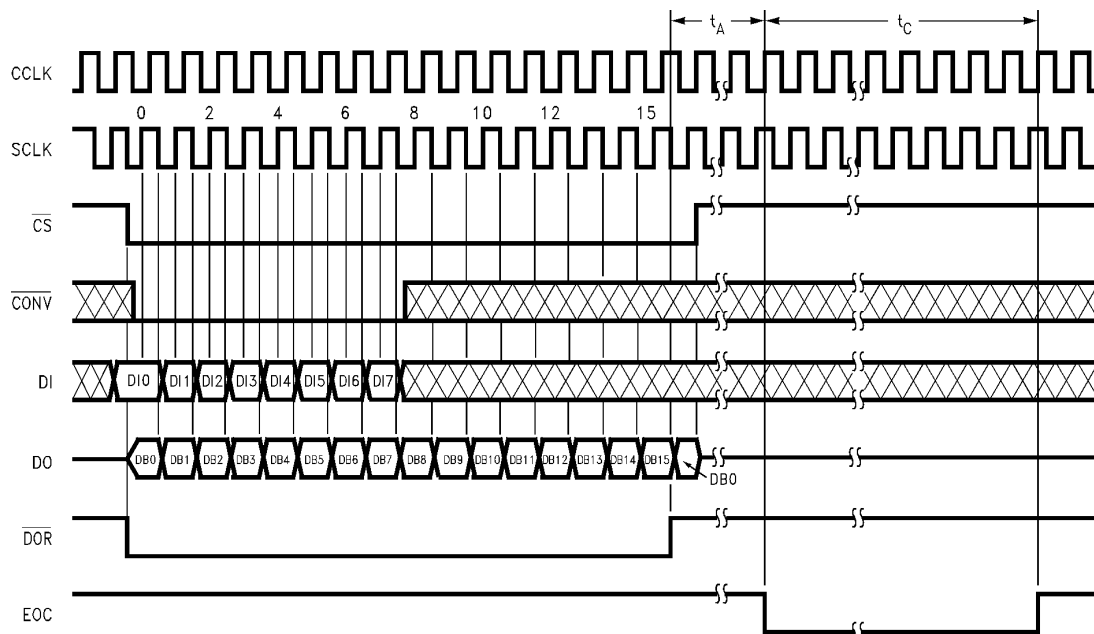
Figure 52. ADC12038 Conversion Using \overline{\text{CS}} with 16-Bit Digital Output Format
