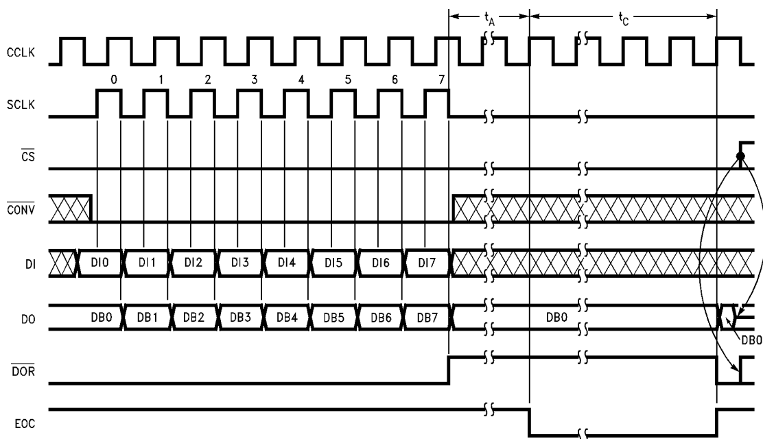
Figure 53. ADC12038 Conversion with \overline{\text{CS}} Continuously Low and 8-Bit Digital Output Format
