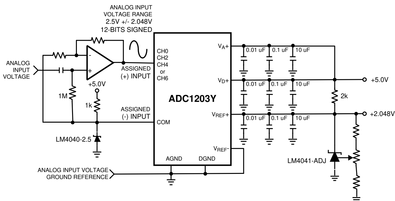
Figure 68. Pseudo-Differential Biasing without the Loss of Digital Output Range
