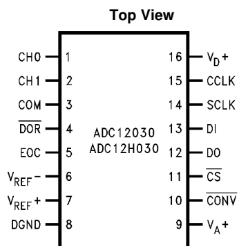
Figure 1. 16-Pin Wide Body SOIC Package See Package Number DW0016B
