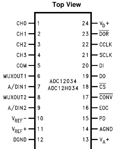
Figure 3. 24-Pin Wide Body SOIC, PDIP, SSOP Packages See Package Numbers DW0024B, NAM0024D, DB0024A
