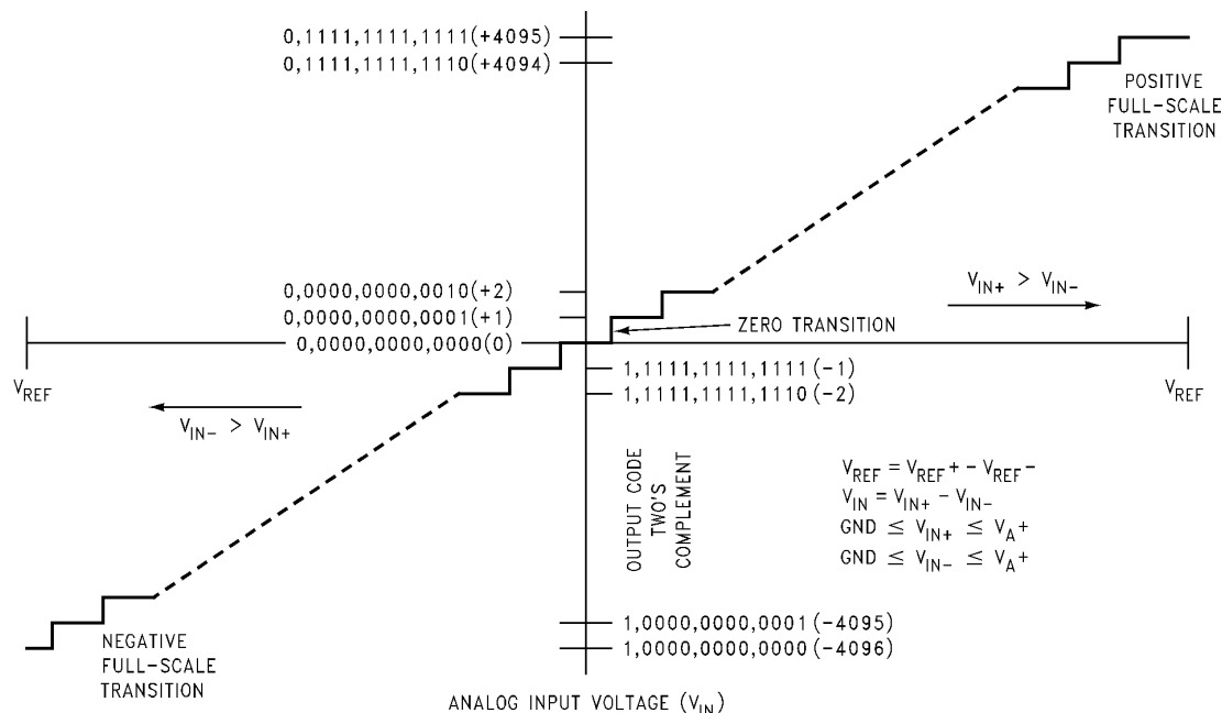
Figure 5. Transfer Characteristic
