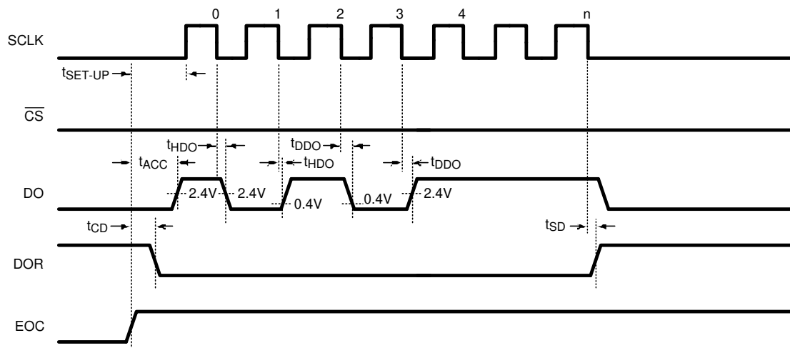
Figure 47. DO Data Output Timing with \overline{\text{CS}} Continuously Low
