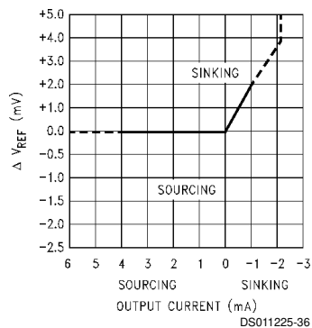
Load Regulation
