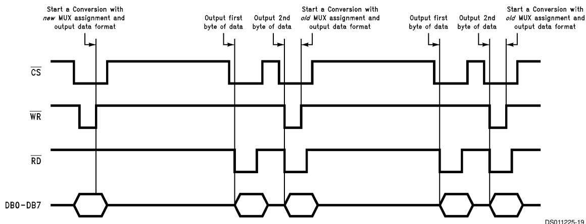
FIGURE 3. Starting a Conversion without Updating the Channel Configuration, Resolution, or Data Format
