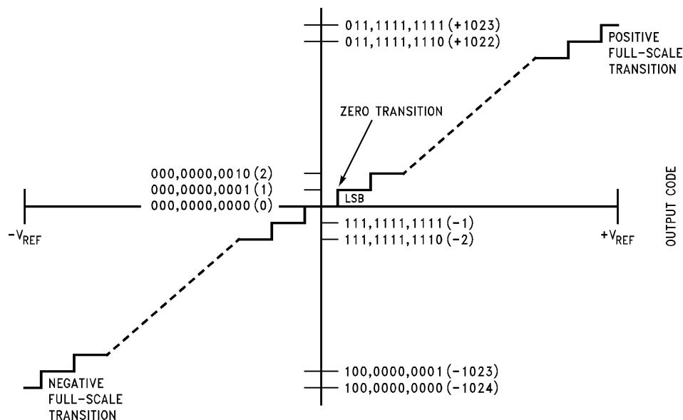
FIGURE 1. Transfer Characteristic
