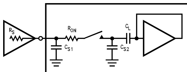
FIGURE 6. Analog Input Model
