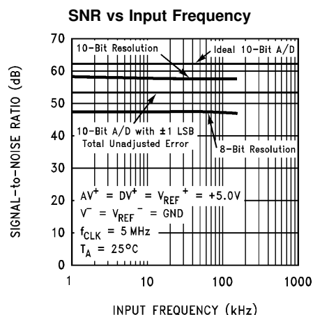
FIGURE 7. ADC10154/ADC10158 Signal-to-Noise Ratio vs Input Frequency
