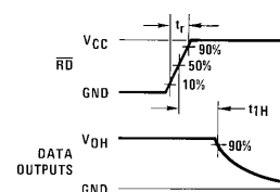
Figure 16. t_{1H} , C_L=10\text{ pF}
