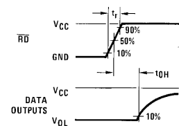
Figure 18. t_{0H} , C_L=10\text{ pF}
