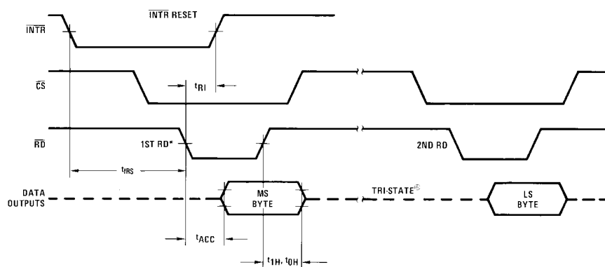
Figure 8. Output Enable and Reset \overline{\text{INTR}}
