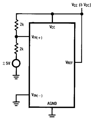
Figure 14. Handling \pm 5\text{V} Analog Inputs
