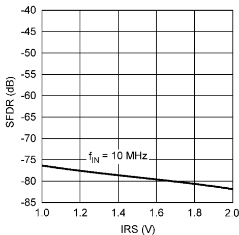
Figure 33. SFDR vs. IRS
