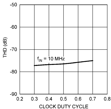
Figure 24. THD vs. Clock Duty Cycle
