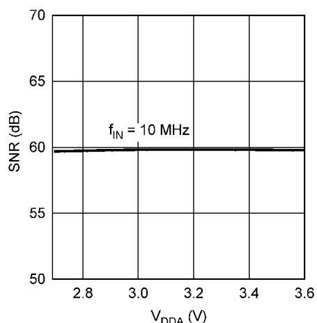
Figure 12. SNR vs. V_{DDA}
