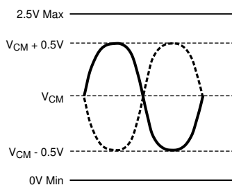
Figure 38. Input Voltage Waveforms for a 2V P-P differential Input
