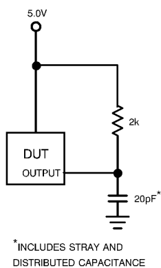
Figure 20. AC Test Circuit
