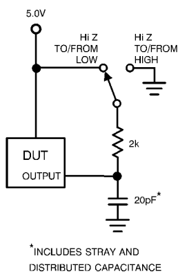
Figure 21. t_{EN} , t_{DIS} Test Circuit
