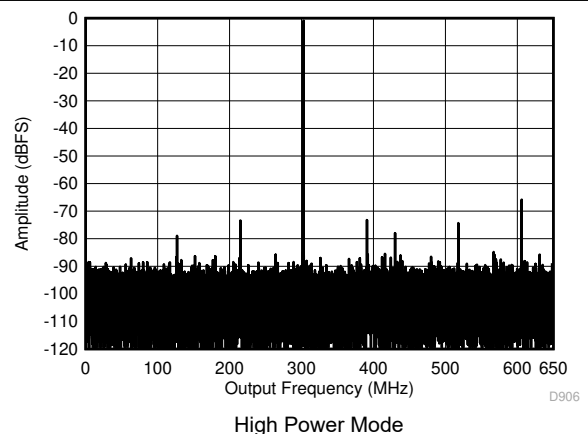
Figure 5-6. Single Tone FFT at 997 MHz and -1 dBFS
