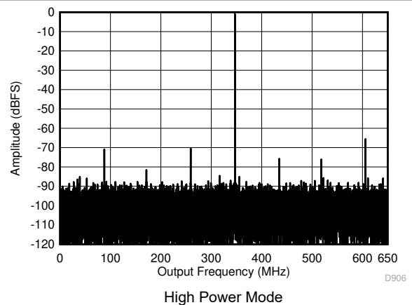
Figure 5-4. Single Tone FFT at 347 MHz and -1 dBFS
