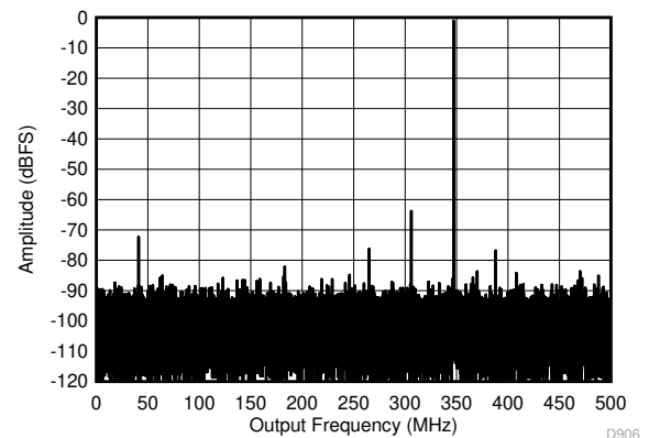
Figure 5-10. Single Tone FFT at 3497 MHz and -1 dBFS
