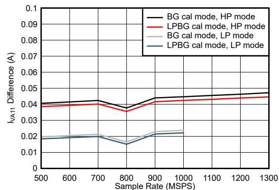
Figure 5-117. Quad Channel, I_{VA11} Change with Calibration Mode
