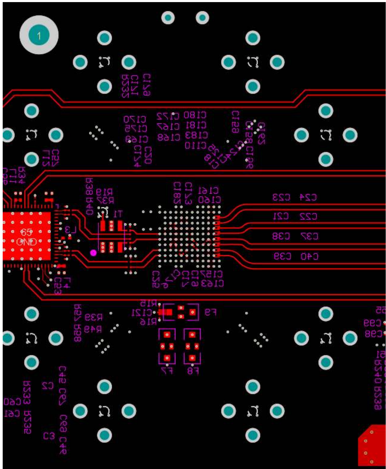
Figure 7-8. Bottom Layer Routing: CLK±, SYSREF and D[7:4]± Routing
