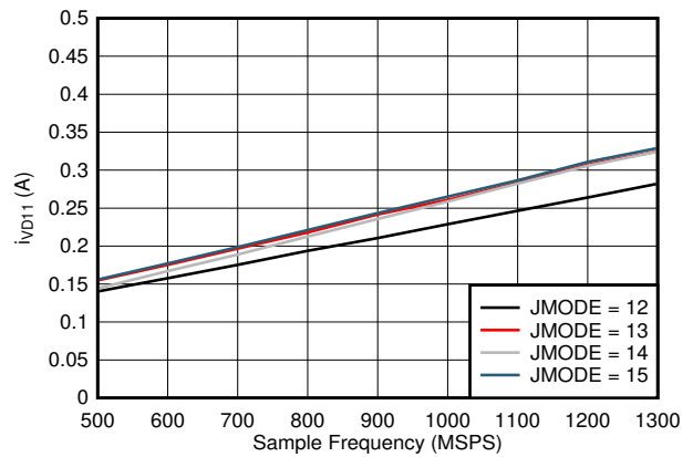
Figure 5-100. Dual Channel, I_{VD11} vs FS and JMODE 12 - 15
