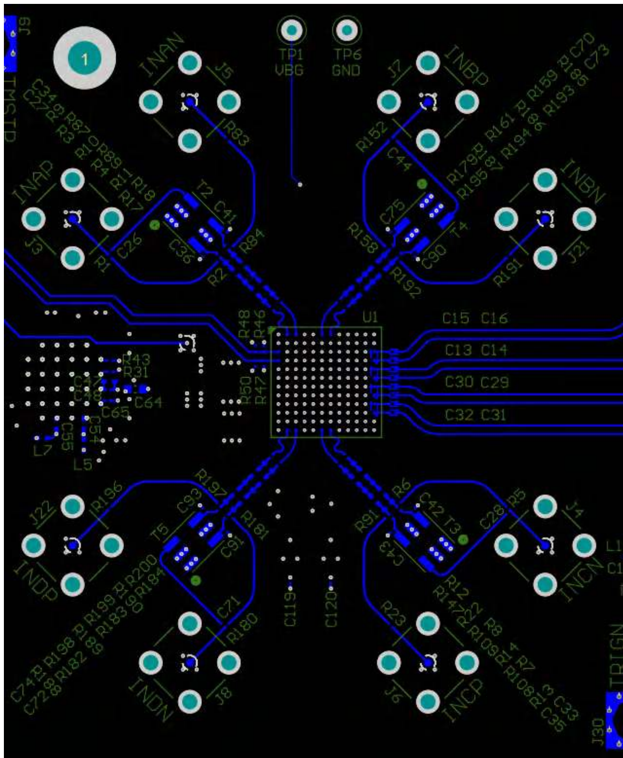
Figure 7-6. Top Layer Routing: Analog Inputs (INA±, INB±, INC±, IND±), TMSTP± and D[3:0]± Routing
