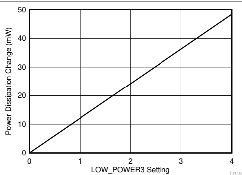
Figure 6-13. Power Dissipation Change vs LOW_POWER3 register setting
