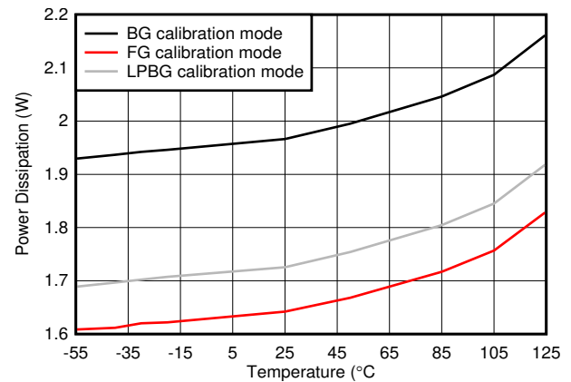
Figure 5-124. Dual Channel, Power Dissipation vs Temperature
