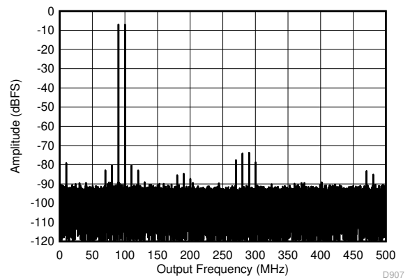
Figure 5-52. Two Tone FFT at 1798 MHz Center
