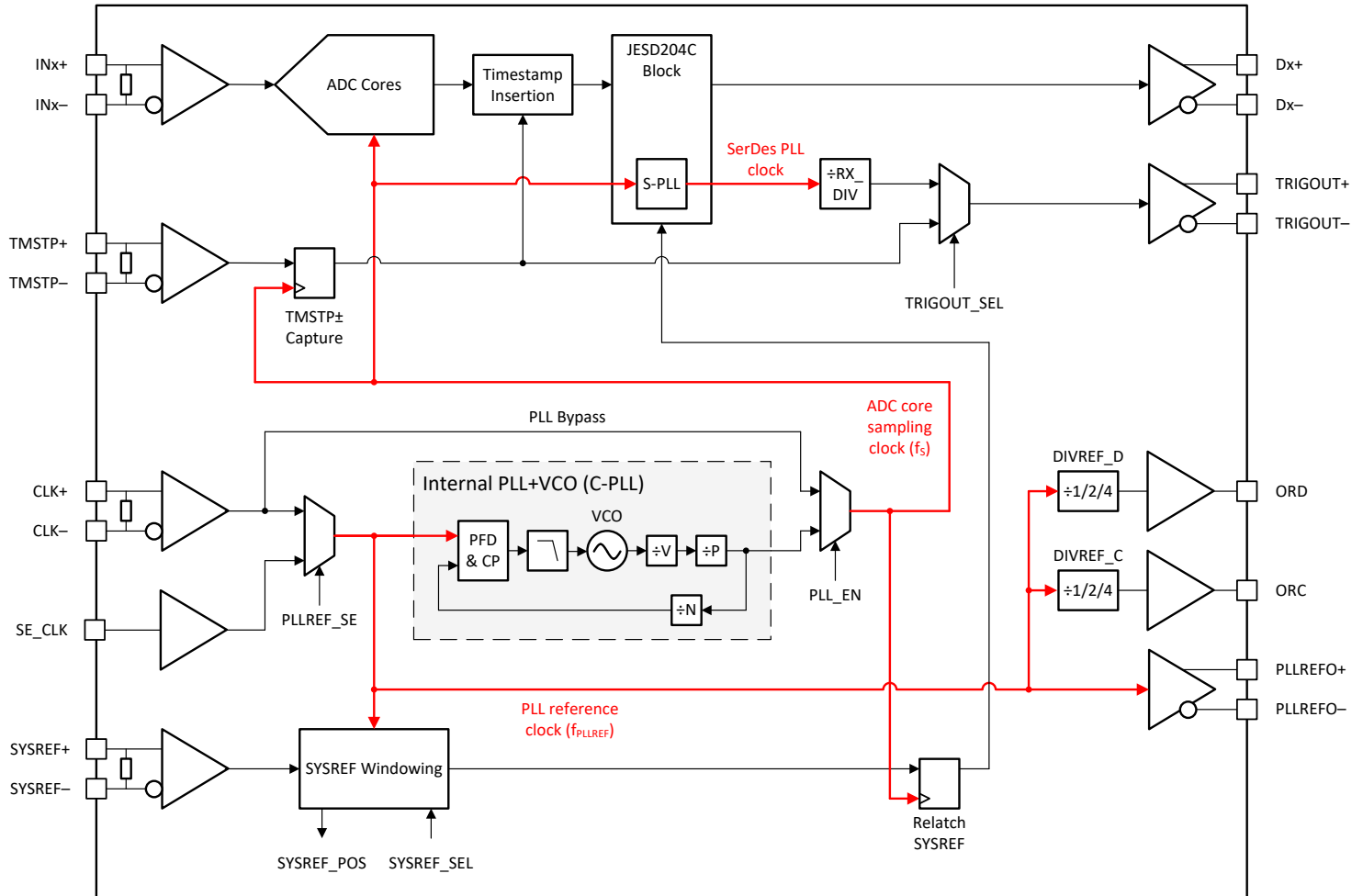
Figure 6-5. Clocking Subsystem
