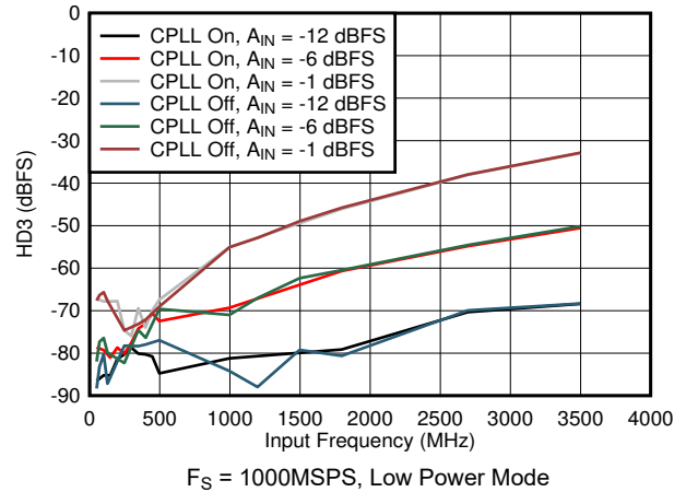
Figure 5-80. HD3 vs Input Frequency, CPLL and Input Amplitude
