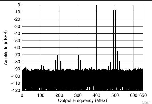
Figure 5-50. Two Tone FFT at 498 MHz Center
