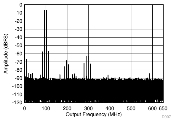
Figure 5-51. Two Tone FFT at 998 MHz Center
