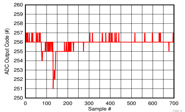
Figure 5-126. Background Calibration Core Transition (midscale voltage)
