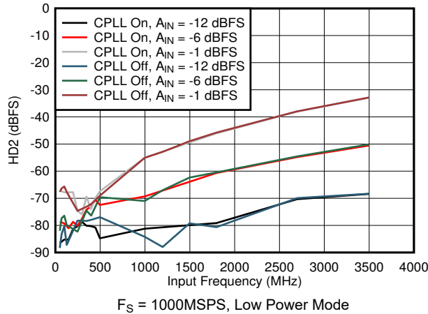
Figure 5-79. HD2 vs Input Frequency, CPLL and Input Amplitude
