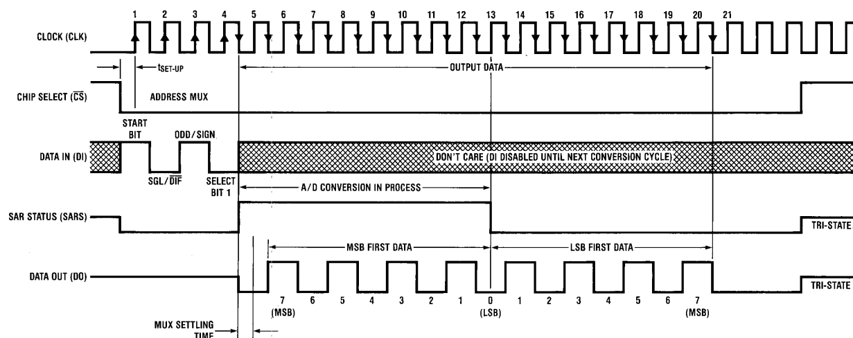
Figure 20. ADC0834-N Timing
