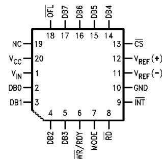
Figure 2. PLCC Package
