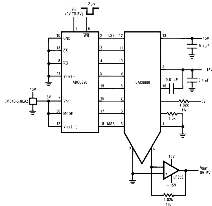
Figure 34. Fast Infinite Sample-and-Hold
