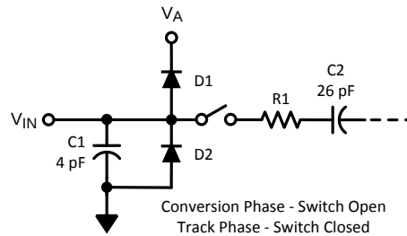
Figure 22. Equivalent Input Circuit
