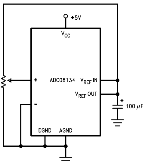
Figure 25. Ratiometric
