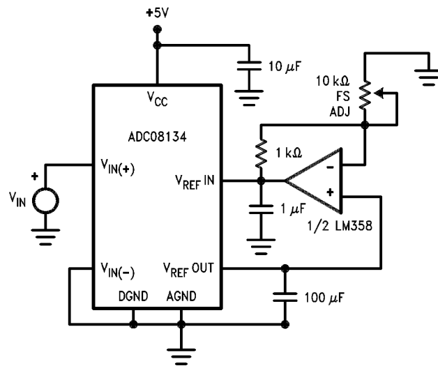
Figure 31. Span Adjust; 0V \leq V_{IN} \leq 3V
