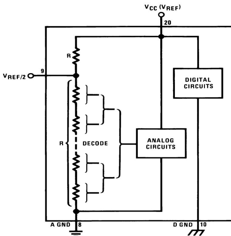
Figure 32. The V_{\text{REFERENCE}} Design on the IC
