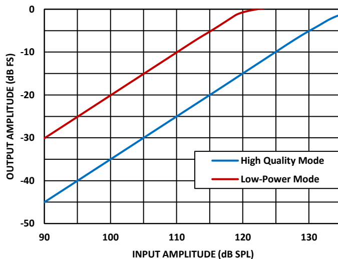
Figure 7. Linearity
