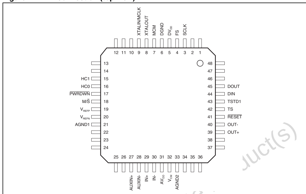
Figure 1. Pin connection (top view)
