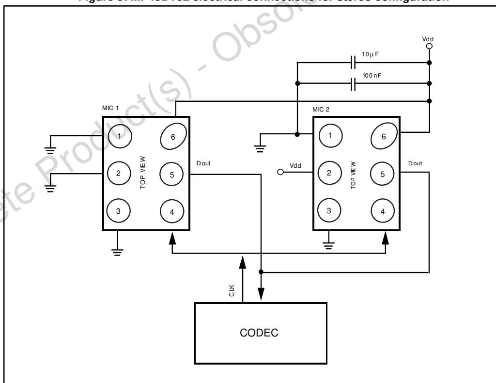
Figure 5: MP45DT02 electrical connections for stereo configuration
