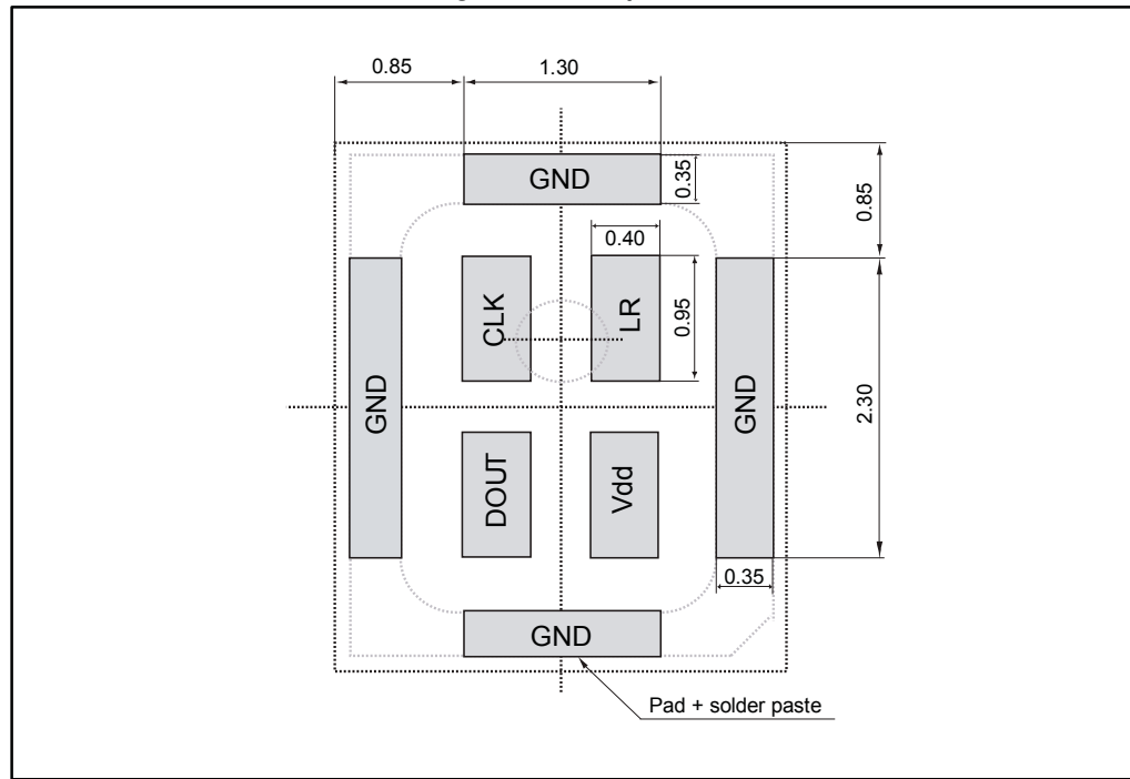
Figure 12: Land pattern
