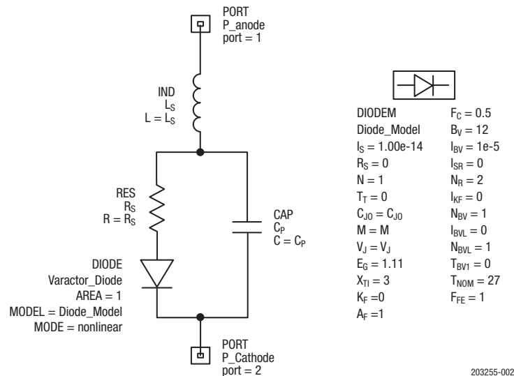
Figure 2. SPICE Model
