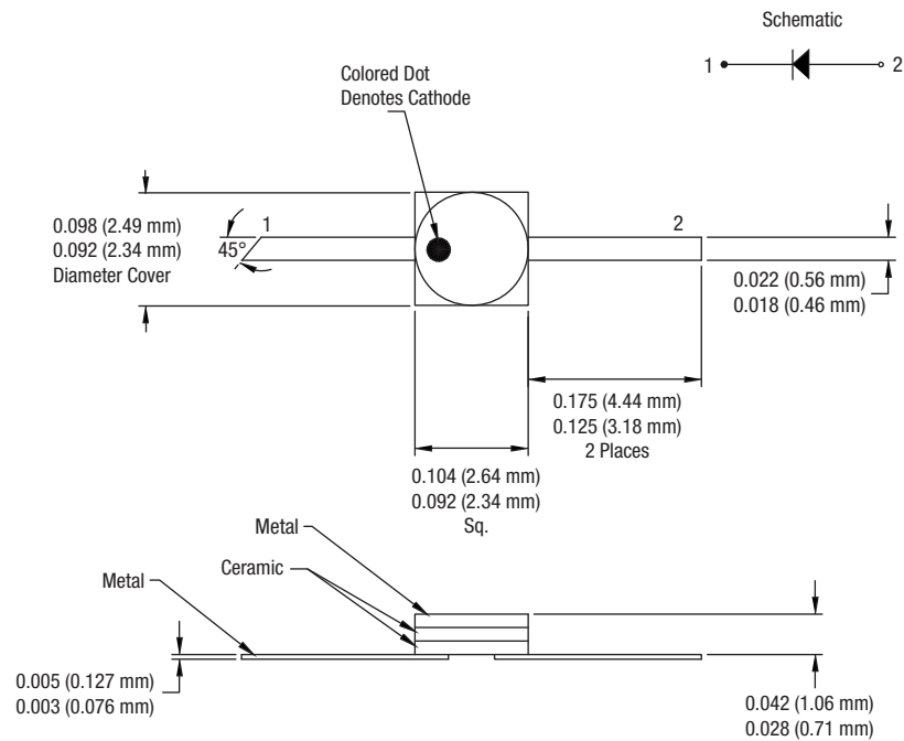
Figure 6. -240 Package Dimensions
