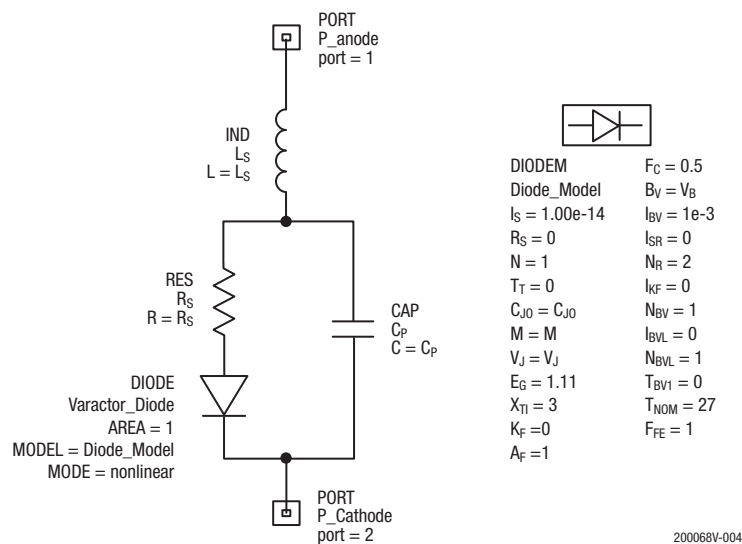
Figure 4. SPICE Model
