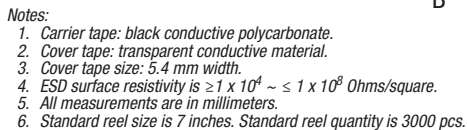
Figure 7. SC-79 Tape and Reel Dimensions
