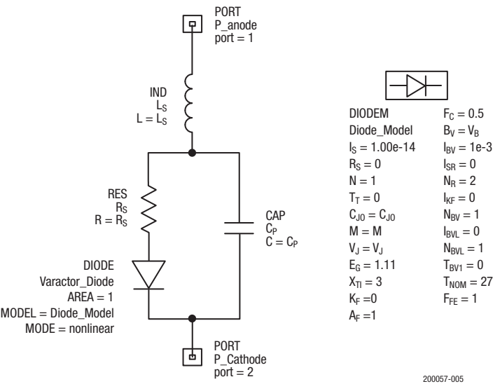
Figure 5. SPICE Model
