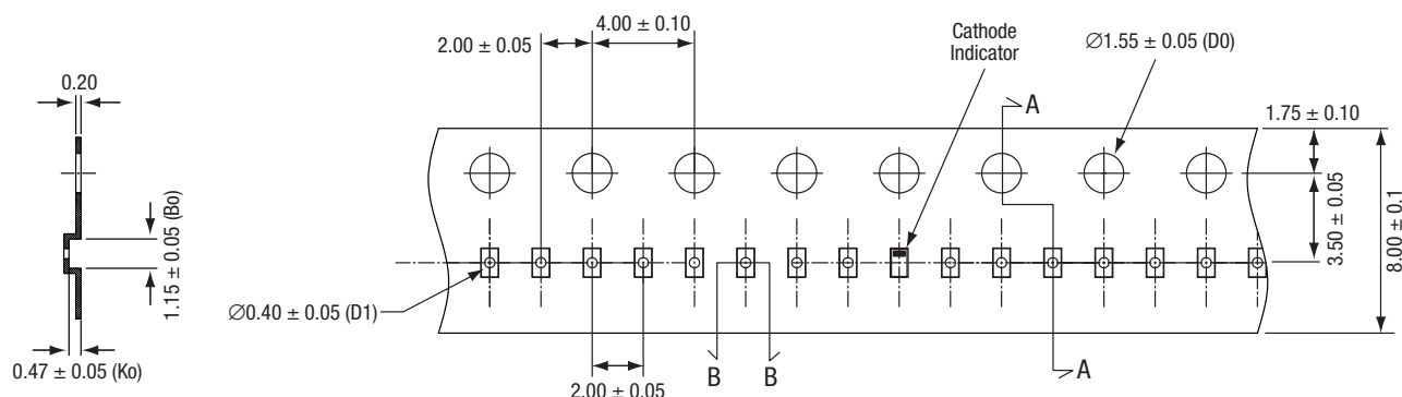
Figure 10. SOD-882 Package Dimensions
