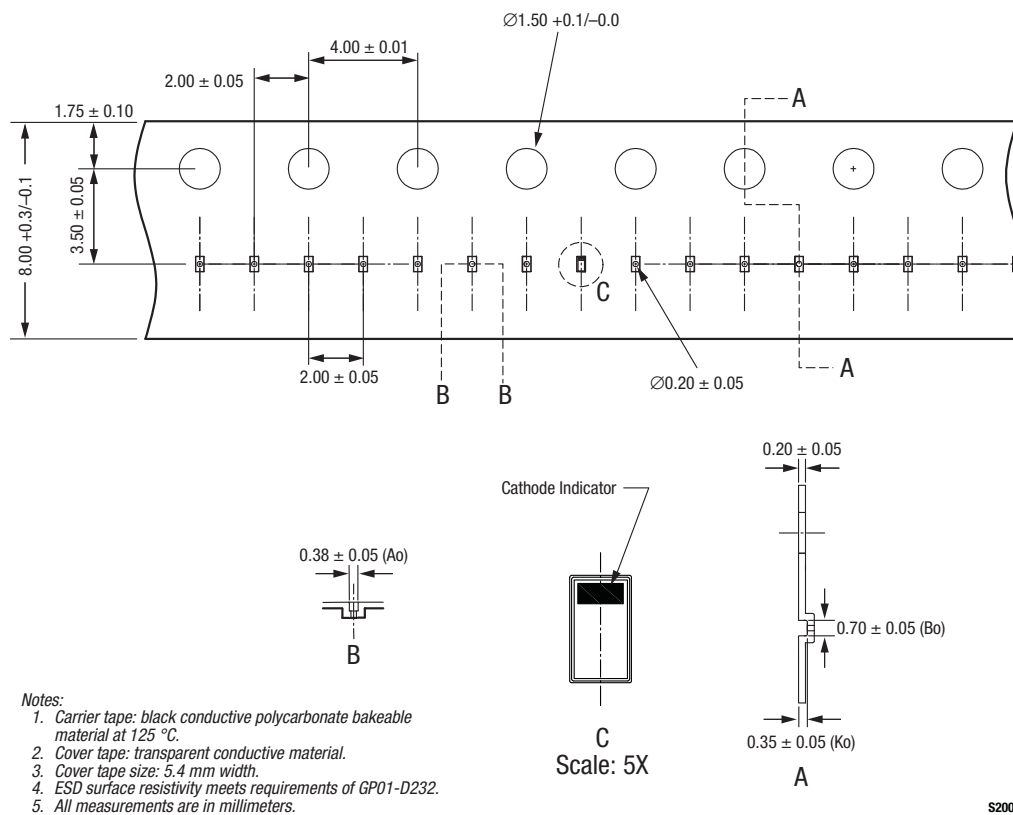
Figure 12. SMSA7621-060 Tape and Reel Dimensions
