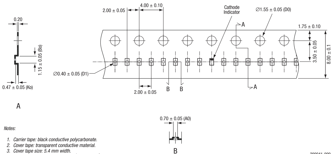
Figure 9. SOD-882 Tape and Reel Dimensions
