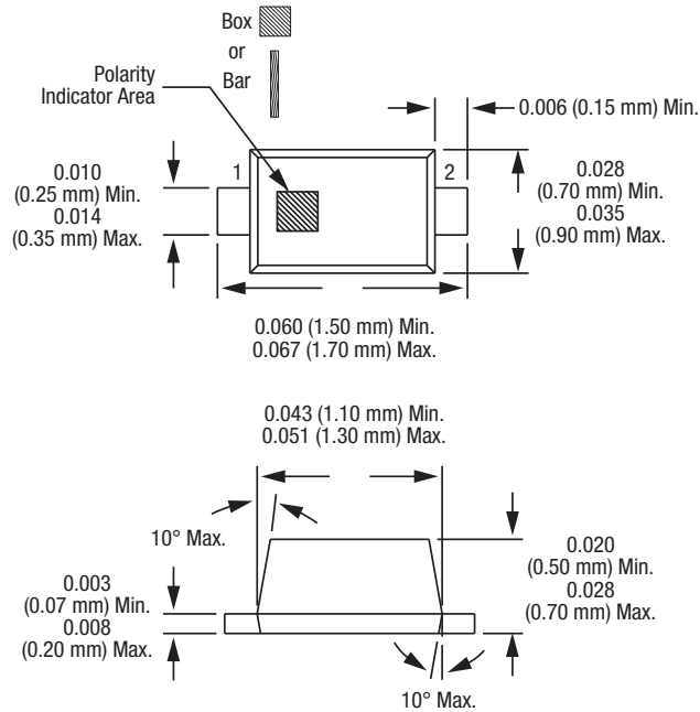
Figure 9. SC-79 Package Dimension Drawing
