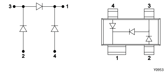
Figure 1. SMPA1304-019LF Package (PI)
