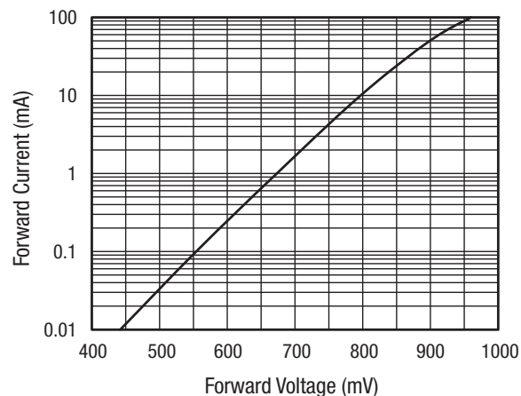
Figure 3. DC Characteristic
