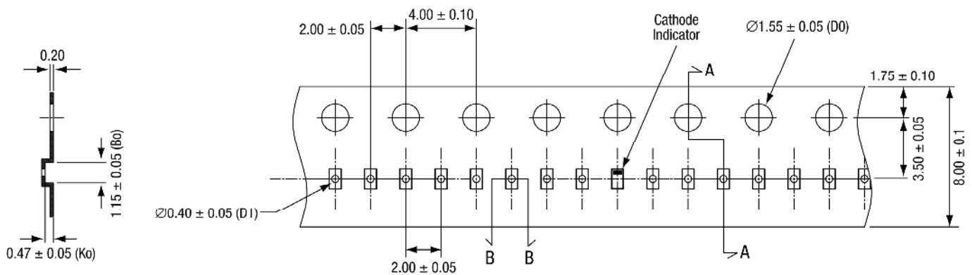
Figure 9. SOD-882 Package Dimension Drawing
