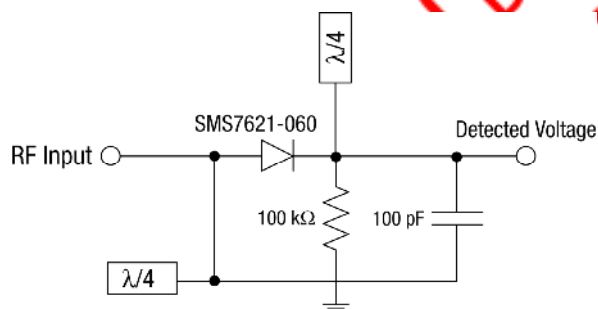
Figure 2. Schematic of a 24 GHz Detector Design
